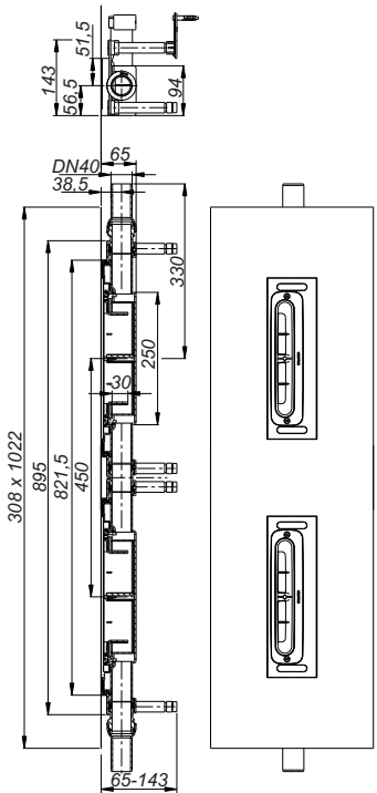
drain body DallFlex Duo Plan
