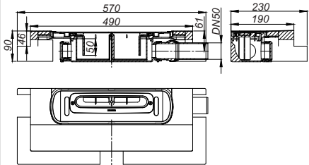
drain body DallFlex EPS assembled
