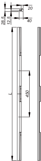
shower channel CeraWall Individual N Duo
