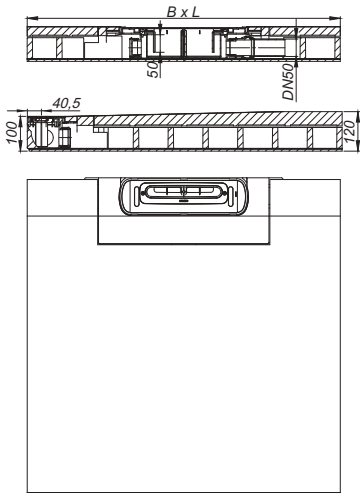
sound-insulating shower underlay DallFlex Wall
