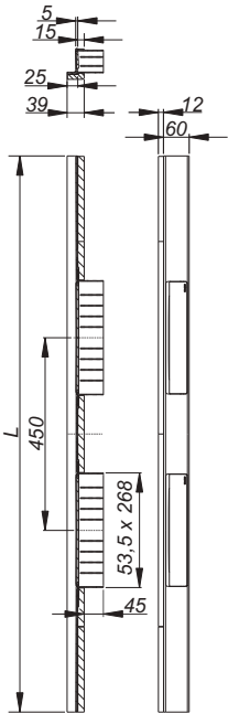
shower channel CeraWall Select N Duo satin stainless steel
