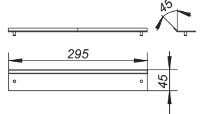
cover plate CeraWall Individual Duo natural stone
