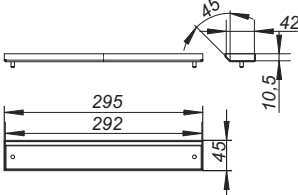
cover plate CeraWall Individual Duo
