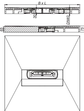
shower underlay DallFlex Compact Plan
