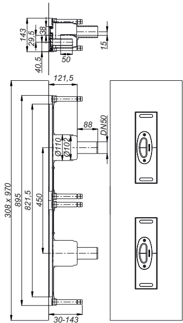
drain body DallFlex Duo vertical
