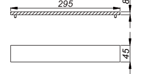
cover plate CeraWall Individual Duo Design
