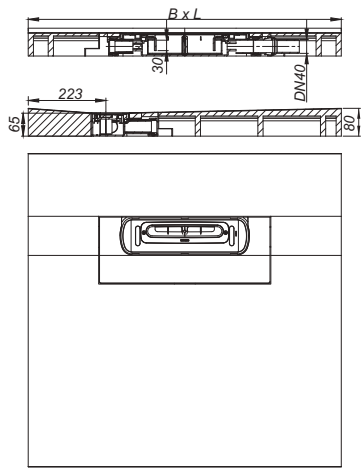
shower underlay DallFlex Floor Plan
