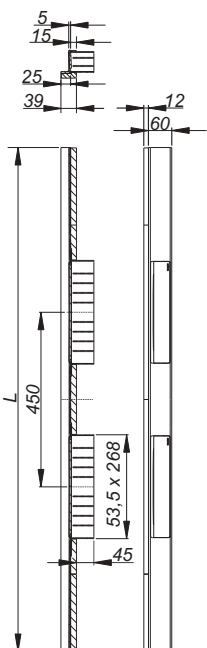
shower channel CeraWall Select N Duo polished stainless steel
